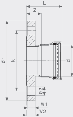
Prestabo XL Flange adapter - galvanised non-alloyed steel Model 1159XL
