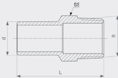
Prestabo Plug-in piece - galvanised non-alloyed steel Model 1111.1
