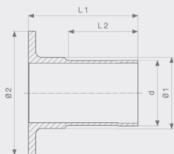
Seapress Flange - CuNiFe Model 0359.3
