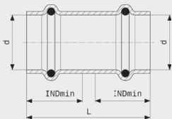
Seapress Sliding coupling - CuNiFe Model 0315.3
