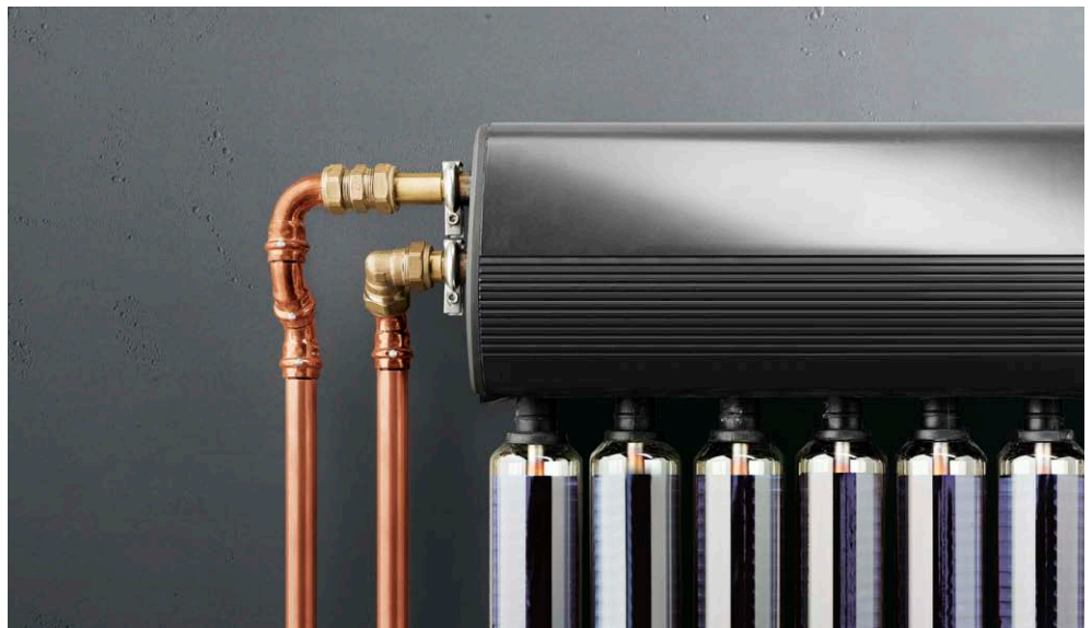
Profipress S on a thermal solar installation with vacuum pipe connectors.
