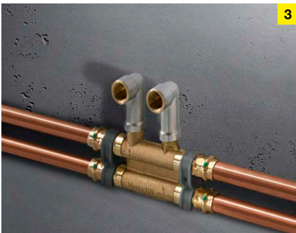
Easy to install: the skirting board radiator connection piece combined with the radiator connection set.
