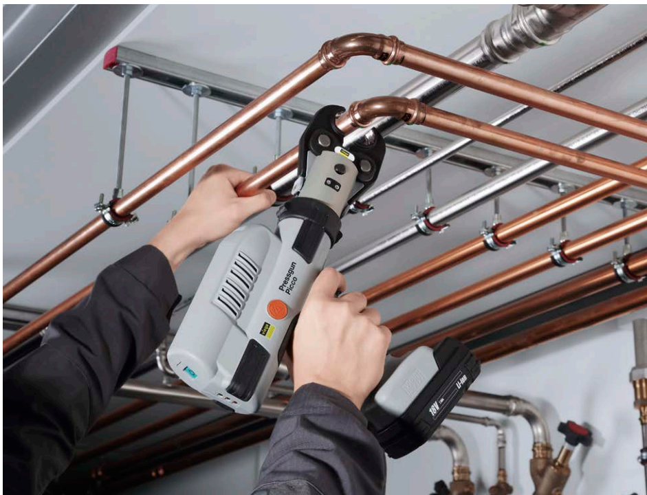
Overhead working – not a problem with Viega Profipress and the single-hand snap action.
