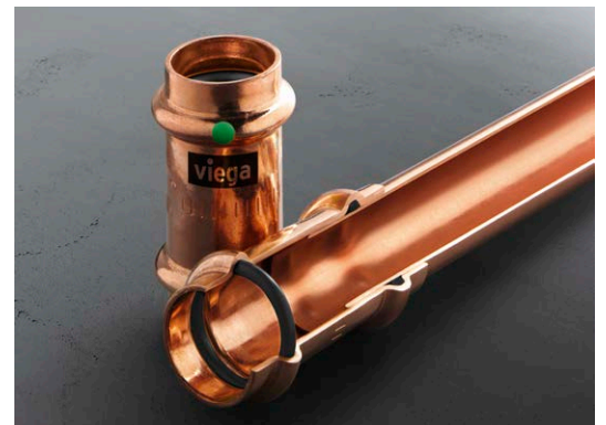
Clear marking: Press connectors marked in green have been factory-fitted with the EPDM sealing element.
