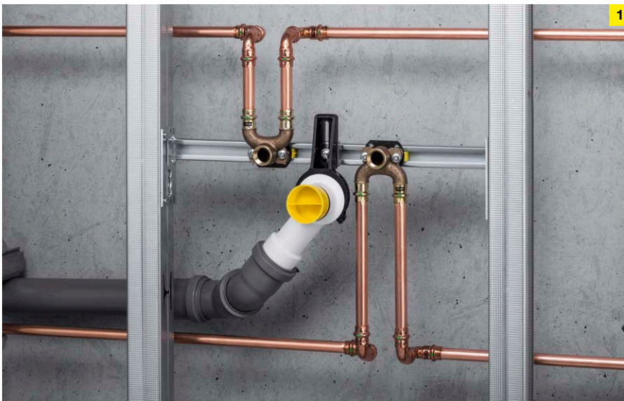
Application example for the connection of double wall plates in ring and series pipeline systems.
