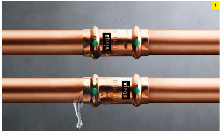
Assured leakage testing with the SC-Contur.
