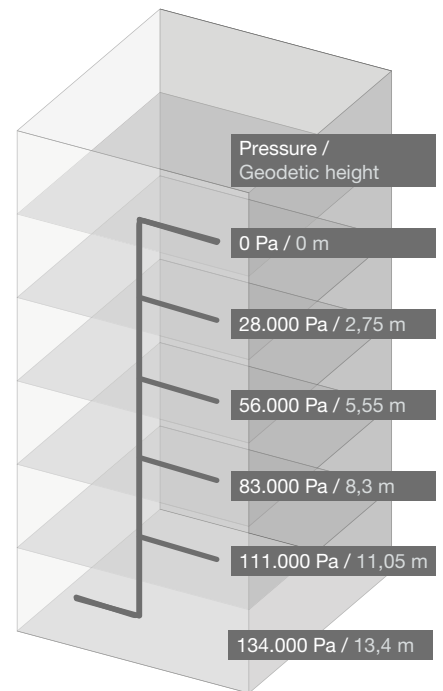
Viega Profipress with SC-Contur ensures forced leakage across the entire pressure testing range.
