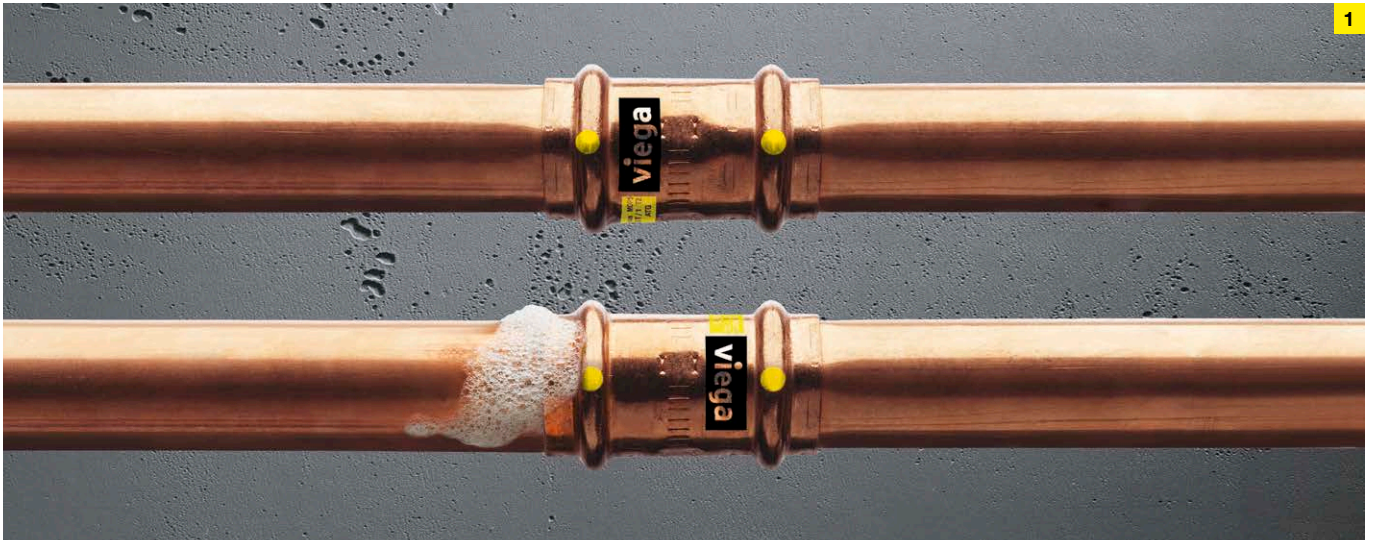
Reliable leakage testing thanks to SC-Contur.
